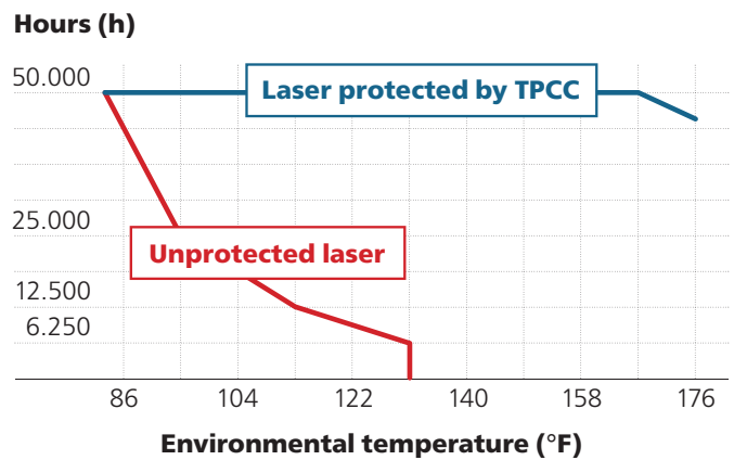
Life-Span of Laser Sensors – Comparison
